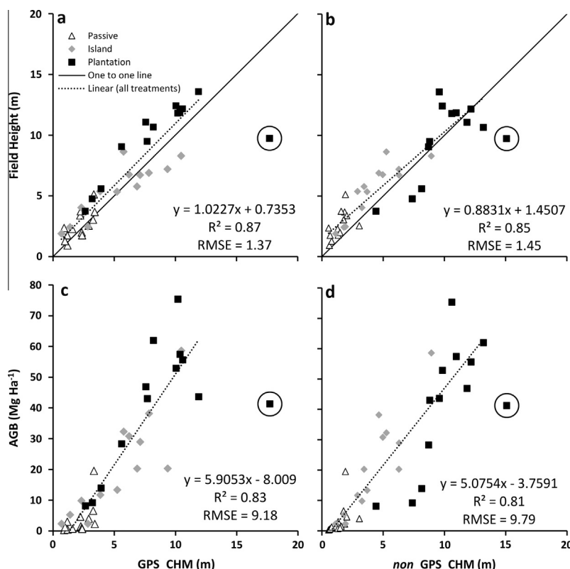
Fig. 2. Median Ecosynth cloud point canopy height models ( GPS\_CHM and non\_GPS\_CHM ) as predictors of field height (a) and (b), and above-ground biomass (AGB) (c) and (d). Regression is for all treatments ( n = 38 points). Circled point is an outlier (Grubbs, 1969) and was not included in analysis.
